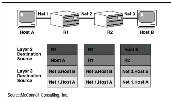
Figure 9: Basic router operations. The sending systems forward the packet to a router which takes over the delivery. Routers calculate the next “hop” and change the Layer 2 address for the next destination. The Layer 3 (network layer) information is unchanged in the IP Datagram.
